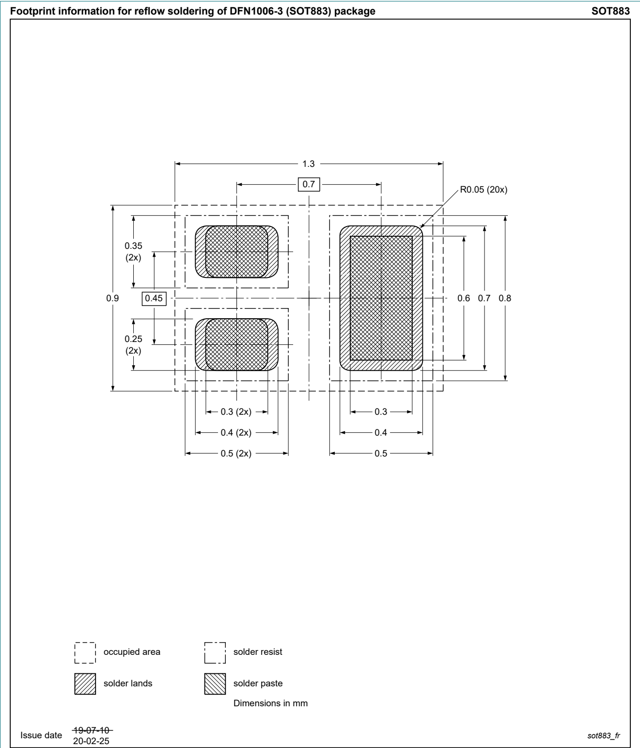
Fig. 19. Reflow soldering footprint for DFN1006-3 (SOT883)
