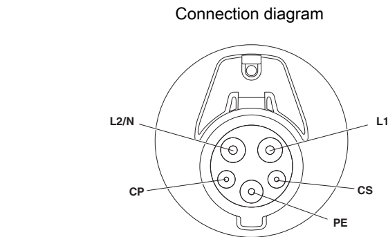
Pin assignment of Vehicle Inlet
