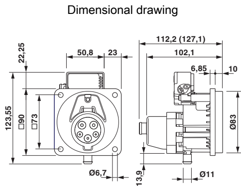
Dimensional drawing
