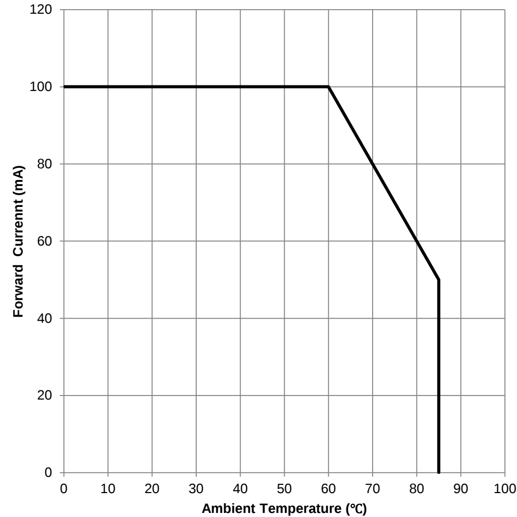
Derating Curve:
