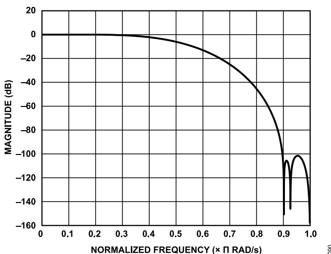
Figure 91. HB3 Filter Response
