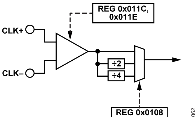
Figure 66. Clock Divider Circuit
