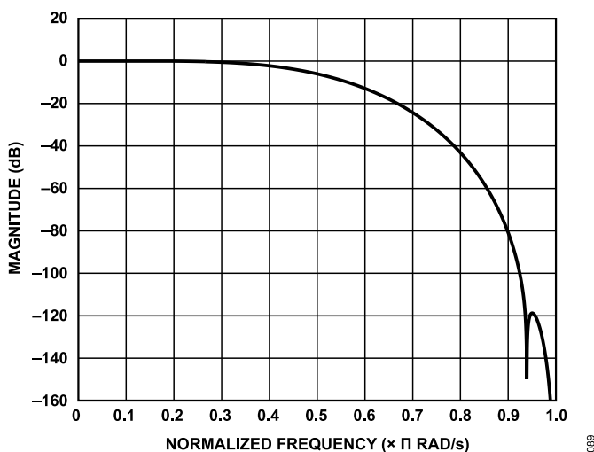
Figure 90. HB4 Filter Response
