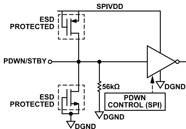
Figure 49. PDWN/STBY Input
