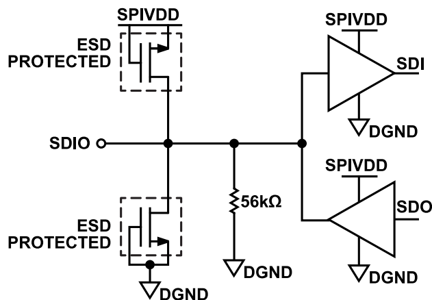
Figure 48. SDIO Input
