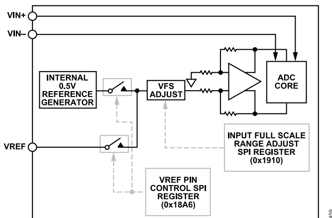
Figure 59. Internal Reference Configuration and Controls
