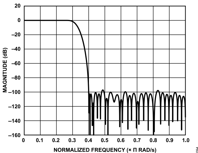
Figure 95. TB1 Filter Response
