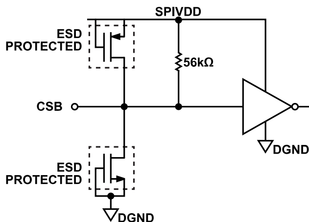
Figure 47. CSB Input
