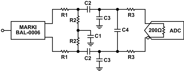
Figure 54. Differential Transformer Coupled Configuration for the AD9699
