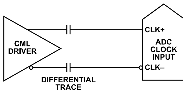
Figure 65. Differential CML Sample Clock
