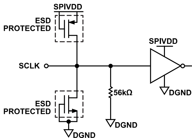
Figure 46. SCLK Input
