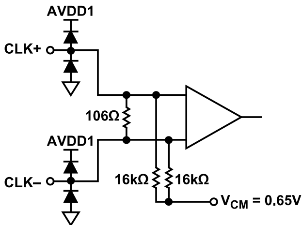
Figure 42. Clock Inputs
