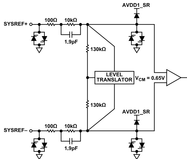
Figure 43. SYSREF± Inputs
