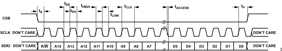
Figure 4. SPI Timing Diagram
