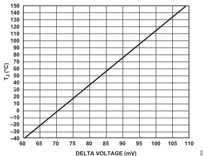
Figure 74. Junction Temperature vs. \Delta V (mV)
