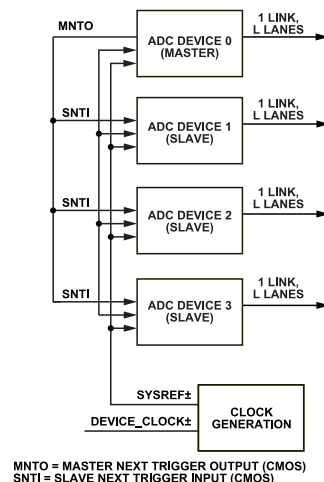
Figure 87. System Using Master/Slave Synchronization Triggering
