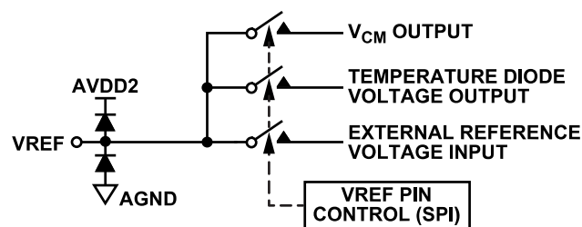
Figure 50. VREF Input/Output
