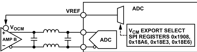
Figure 56. DC-Coupled Application Using the AD9699
