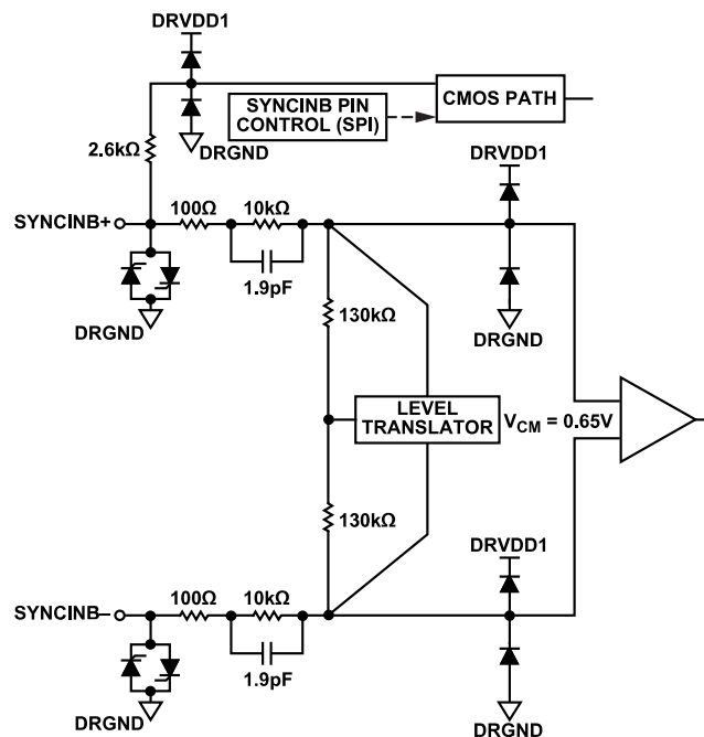
Figure 45. SYNCINB± Inputs
