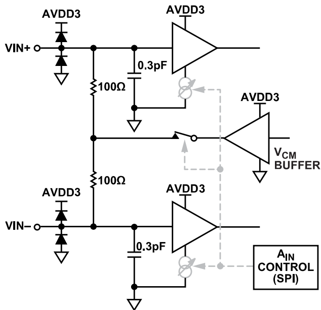
Figure 41. Analog Inputs
