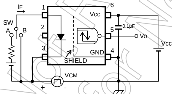
Figure 9: Common-Mode Transient Immunity Test Circuit
