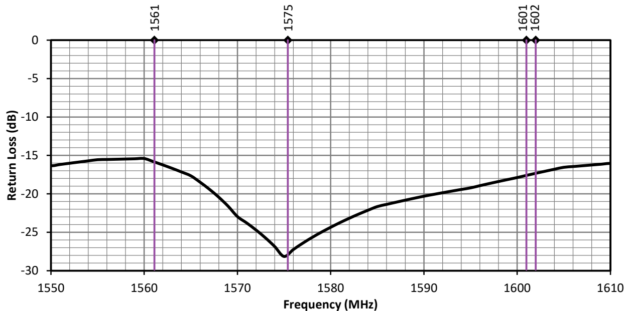
Figure 4. ANT-GNCP-C25L125100 Return Loss, L1 Bands
