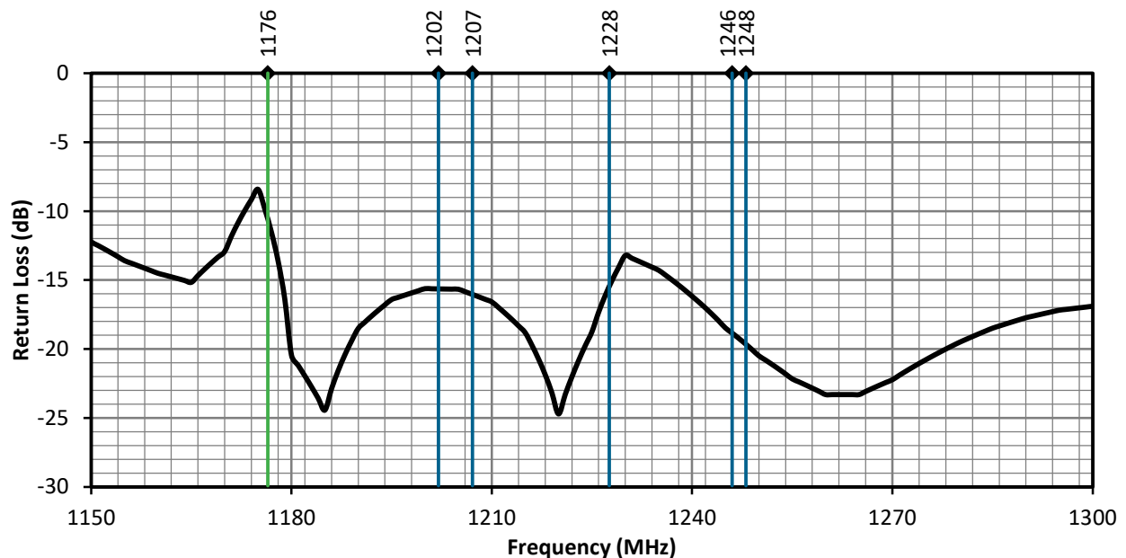
Figure 5. ANT-GNCP-C25L125100 Return Loss, L2 and L5 Bands
