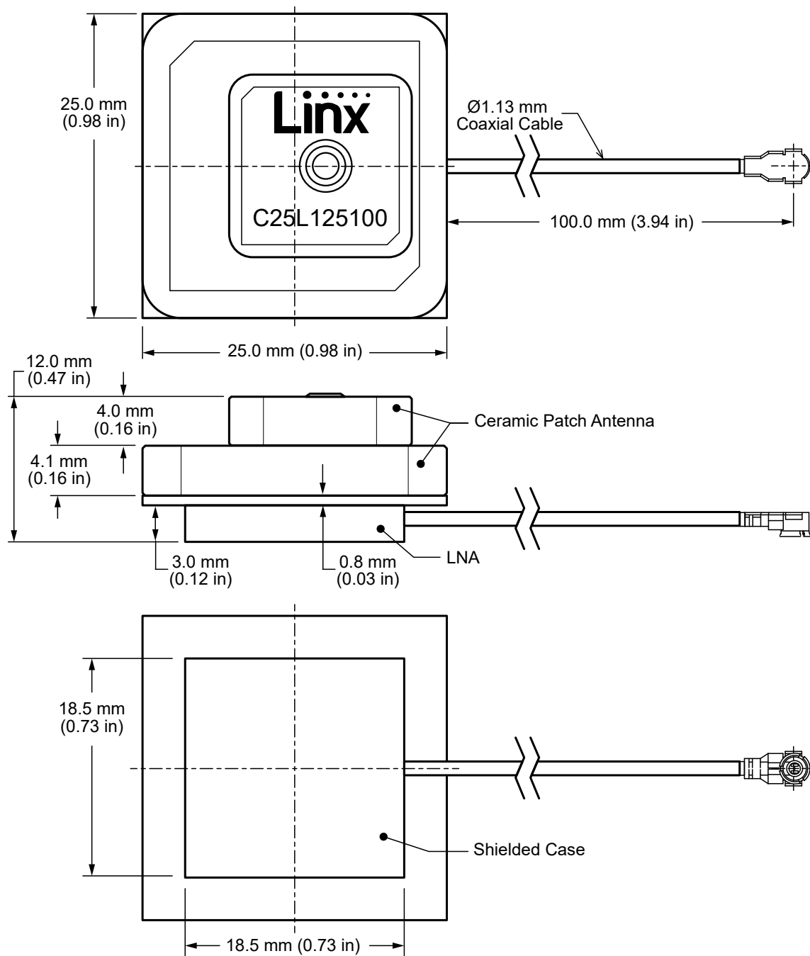
Figure 1. ANT-GNCP-C25L125100 Antenna Dimensions
