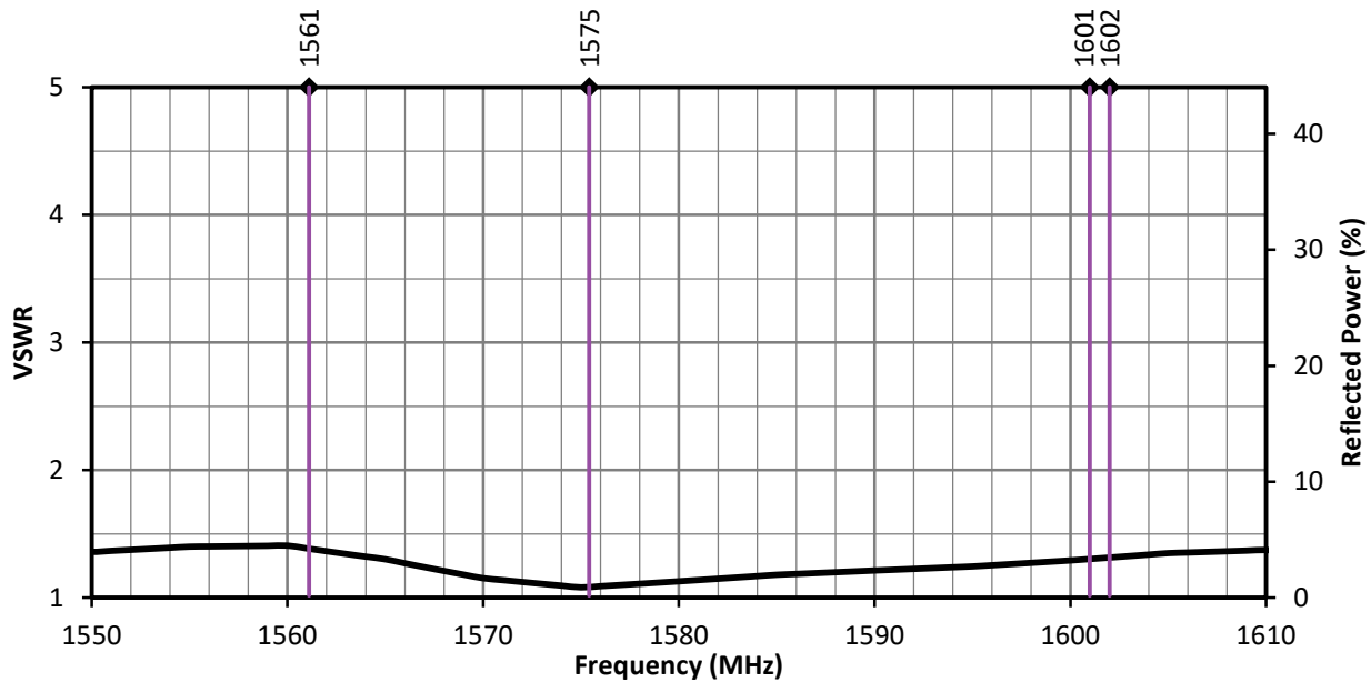
Figure 2. ANT-GNCP-C25L125100 VSWR, L1 Bands
