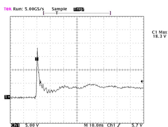
Fig. 6 - ESD Clamping Voltage
