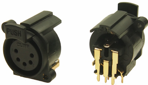
CP300405 - 5XNACF/PC90L Female 5 Pin 90 deg. PCB mount with latch.
