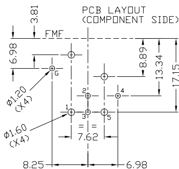
CP300405 - 5XNACF/PC90L Female 5 Pin 90 deg. PCB mount with latch.
