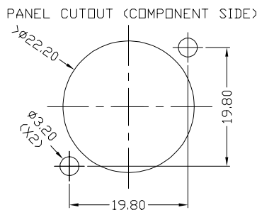
CP300405 - 5XNACF/PC90L Female 5 Pin 90 deg. PCB mount with latch.
