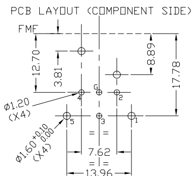
CP300255 - 5XNACM/PC90 Male 5 Pin 90 deg. PCB mount.
