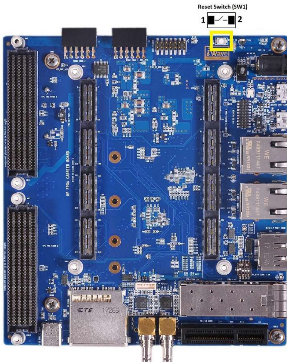
Figure 25: Reset Switch
