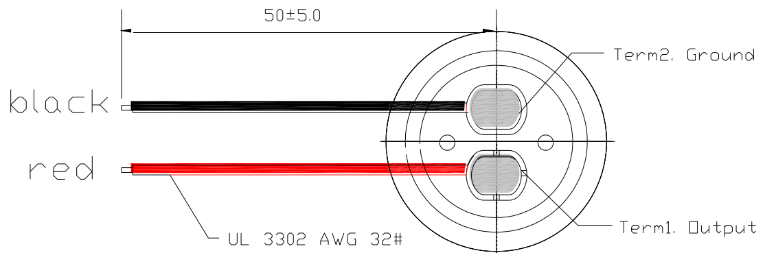
BOTTOM VIEW
