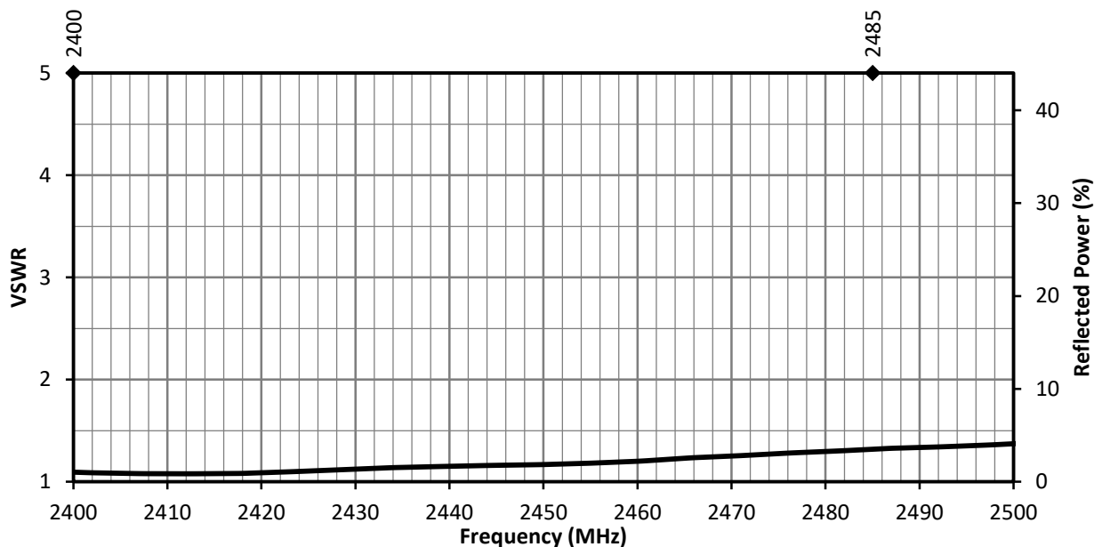
Figure 2. ANT-2.4-FPC-LH Antenna VSWR
