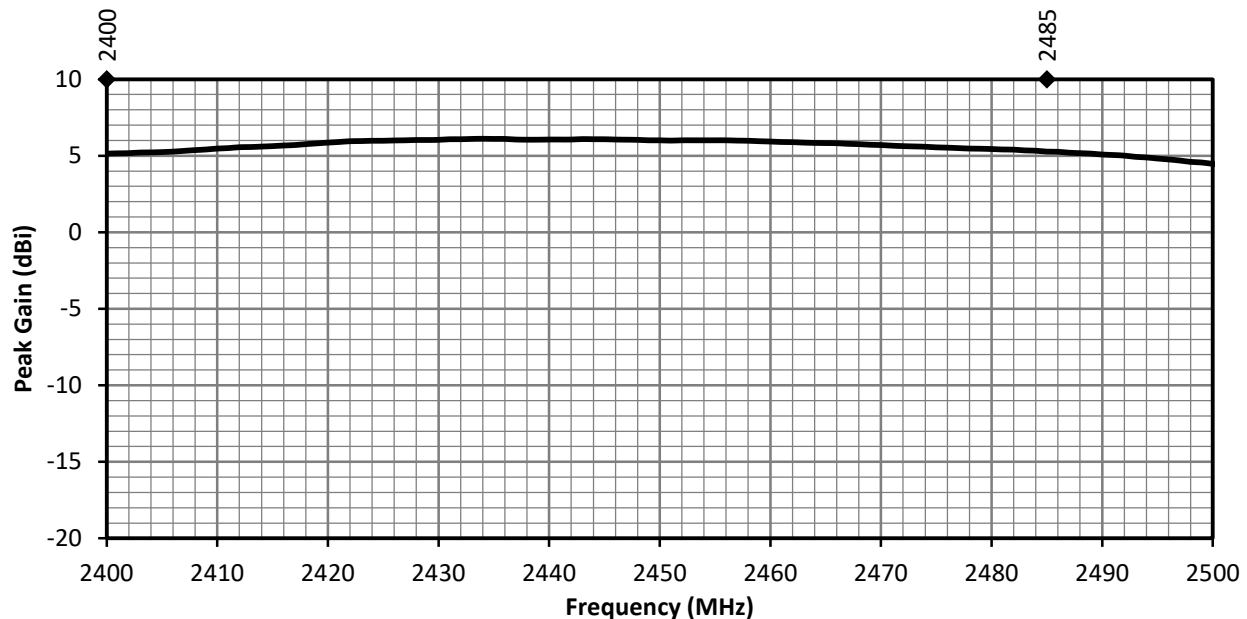
Figure 4. ANT-2.4-FPC-LH Antenna Peak Gain
