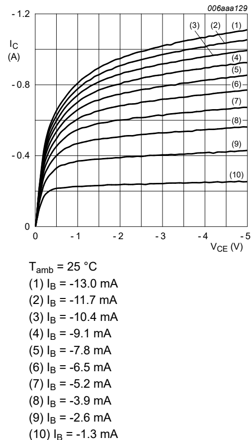
Fig. 9. BC807-25QB-Q: Collector current as a function of collector-emitter voltage; typical values
