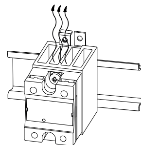
Fig. 13 Mount heatsink with fins in the vertical orientation to guarantee the best possible airflow through the heatsink.
