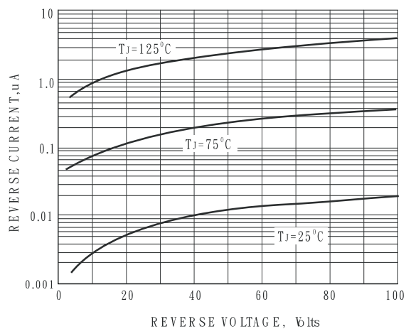
FIG.2-TYPICAL REVERSE CHARACTERISTICS
