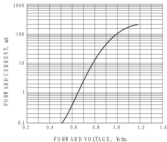
FIG. 1-TYPICAL FORWARD CHARACTERISTIC
