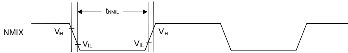
NMIX Input Timing
