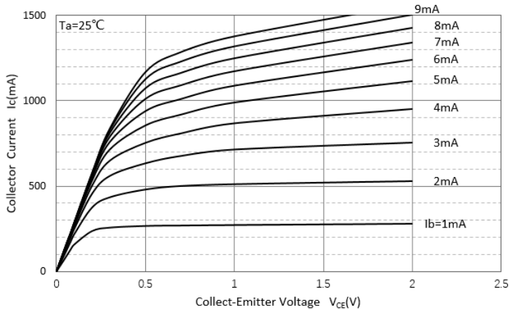
Static Characteristic
