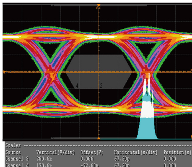
48" Input, EQ=10dB, 500mV Swing, Pre-emp=0dB, Rout_S0=1
