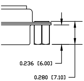
3 ..... 0.236" MATING SIDE
