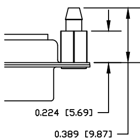
5 ..... 0.224" PCB SIDE
