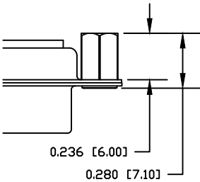
2 ..... 0.236" PCB SIDE
