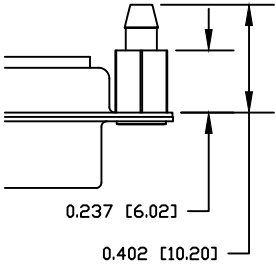
4 ..... 0.237" PCB SIDE
