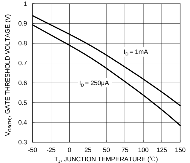
Figure 8. Gate Threshold Voltage vs. Junction Temperature
