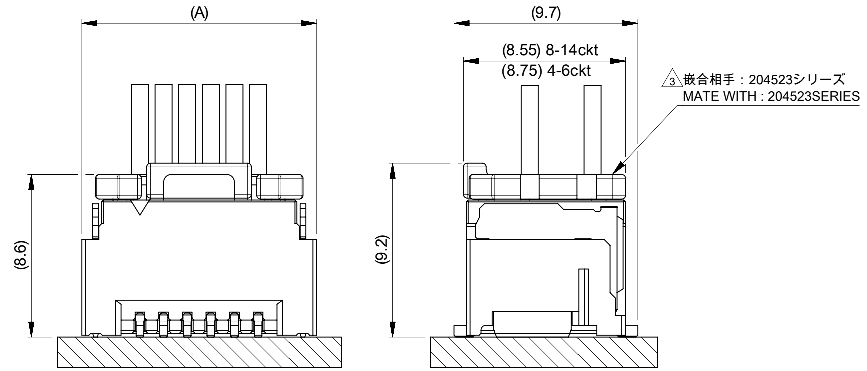
3 嵌合図 MATED CONNECTORS
