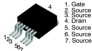
D2PAK7 (TO-263 7 LD) CASE 418AY
