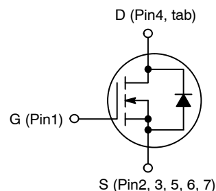
N-Channel MOSFET
