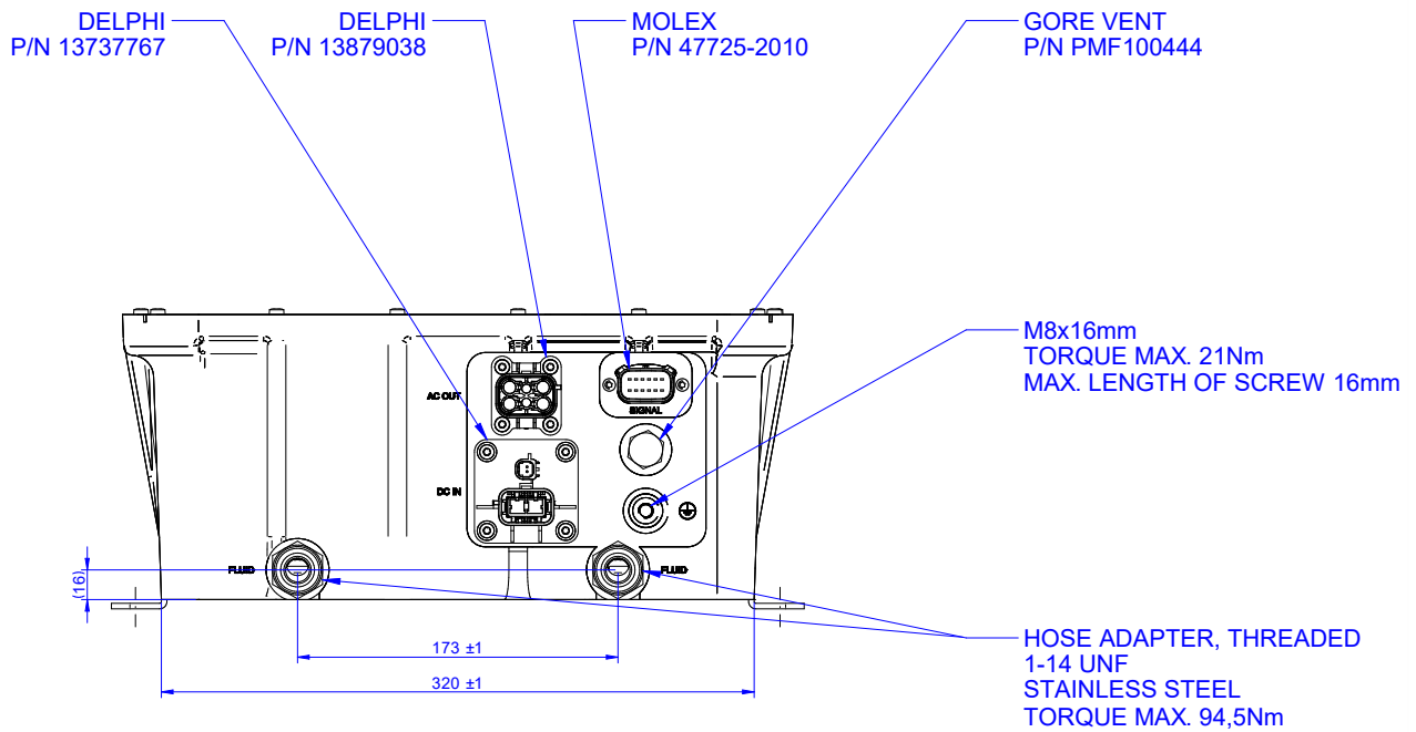
Figure 5. Front view
