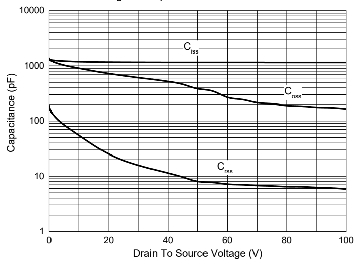
Fig. 7 - Capacitance Characteristics
