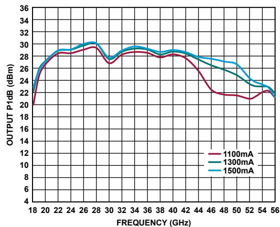
Figure 62. Output P1dB vs. Frequency for Various Supply Currents, V_{DD} = 4\text{ V}
