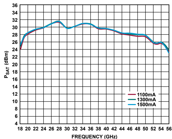
Figure 63. P_{SAT} vs. Frequency for Various Supply Currents, V_{DD} = 4\text{ V}
