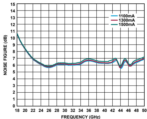
Figure 64. Noise Figure vs. Frequency for Various Supply Currents, V_{DD} = 4\text{ V}
