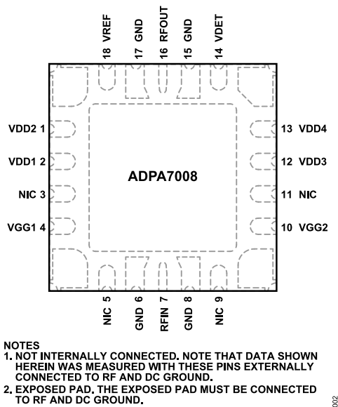
Figure 2. Pin Configuration
