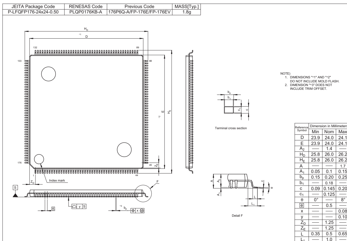
Figure 1.3 176-pin LQFP
