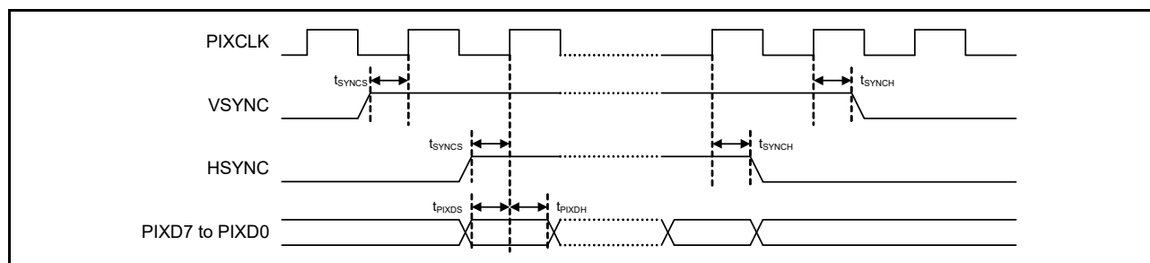
Figure 2.72 PDC AC timing
