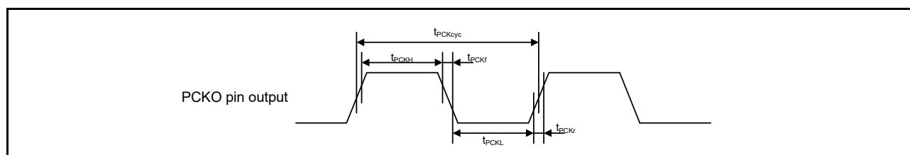
Figure 2.71 PDC output clock timing
