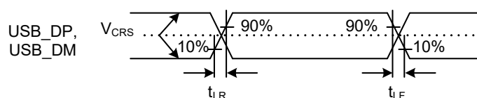
Figure 2.84 USB_DP and USB_DM output timing in low-speed mode
