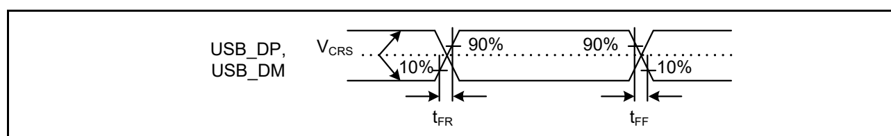
Figure 2.86 USB_DP and USB_DM output timing in full-speed mode
