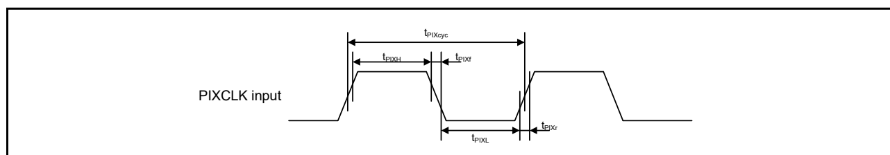
Figure 2.70 PDC input clock timing
