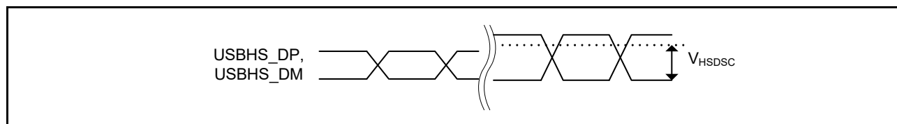
Figure 2.81 USBHS_DP and USBHS_DM disconnect detect sensitivity in high-speed mode
