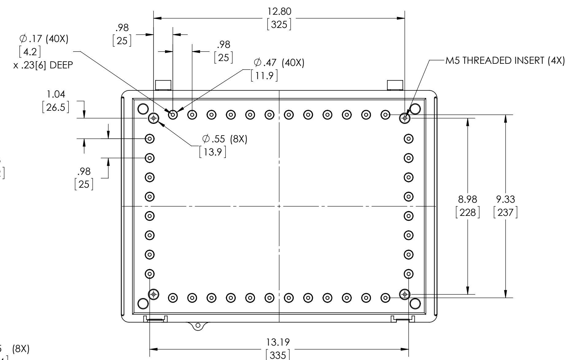
INSIDE VIEW OF BODY
