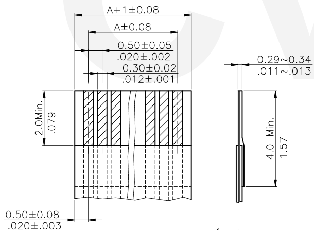
Accommodated FFC/FPC
