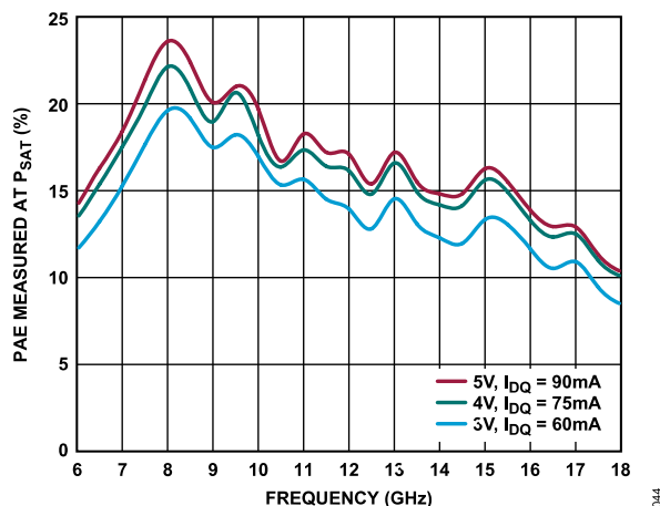
Figure 44. PAE Measured at P_{SAT} vs. Frequency for Various Supply Voltages and I_{DD} , R_{BIAS} = 4.12\text{ k}\Omega
