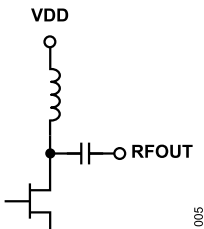
Figure 5. VDD and RFOUT Interface Schematic
