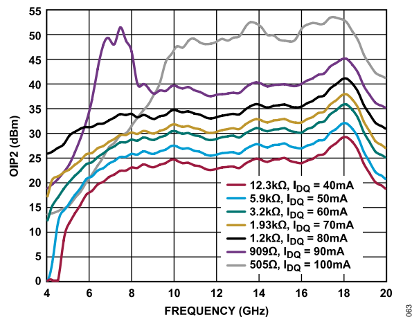
Figure 63. OIP2 vs. Frequency for R_{BIAS} Values and Various I_{DQ} , V_{DD} = 3\text{ V}
