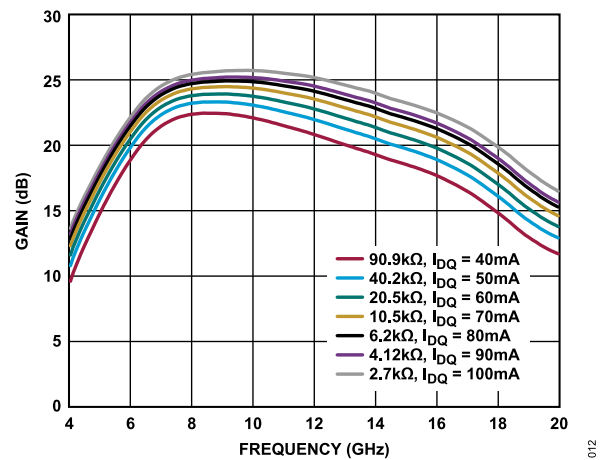
Figure 12. Gain vs. Frequency for R_{BIAS} Values and Various I_{DQ} , V_{DD} = 5\text{ V}
