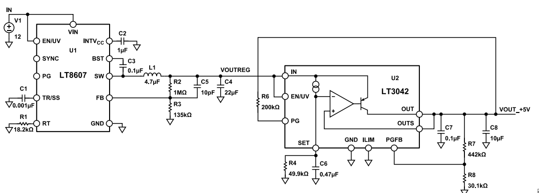
Figure 82. Recommended Power Management Circuit
