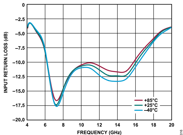
Figure 16. Input Return Loss vs. Frequency for Various Temperatures, 4 GHz to 20 GHz, V_{DD} = 5\text{ V} , I_{DQ} = 90\text{ mA} , R_{BIAS} = 4.12\text{ k}\Omega
