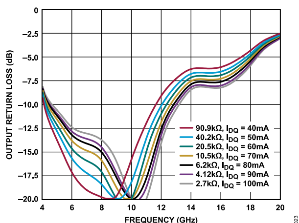
Figure 23. Output Return Loss vs. Frequency for R_{BIAS} Values and Various I_{DQ} , V_{DD} = 5\text{ V}
