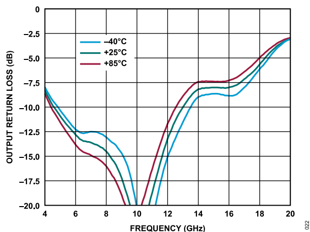
Figure 22. Output Return Loss vs. Frequency for Various Temperatures, 4 GHz to 20 GHz, V_{DD} = 5\text{ V} , I_{DQ} = 90\text{ mA} , R_{BIAS} = 4.12\text{ k}\Omega
