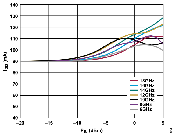
Figure 54. I_{DD} vs. P_{IN} for Various Frequencies, V_{DD} = 5\text{ V} , R_{BIAS} = 4.12\text{ k}\Omega
