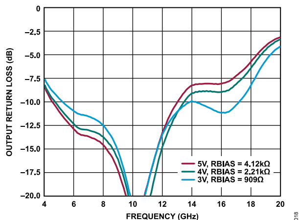
Figure 18. Output Return Loss vs. Frequency for Various Supply Voltages and R_{BIAS} Values, I_{DQ} = 90\text{ mA}
