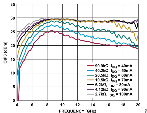
Figure 59. OIP3 vs. Frequency for R_{BIAS} Values and Various I_{DQ} , V_{DD} = 5\text{ V}
