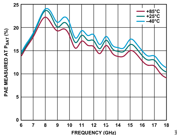
Figure 46. PAE Measured at P_{SAT} vs. Frequency for Various Temperatures, 6 GHz to 18 GHz, V_{DD} = 5\text{ V} , I_{DD} = 90\text{ mA} , R_{BIAS} = 4.12\text{ k}\Omega
