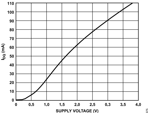
Figure 75. I_{DQ} vs. Supply Voltage, R_{BIAS} = 909\ \Omega
