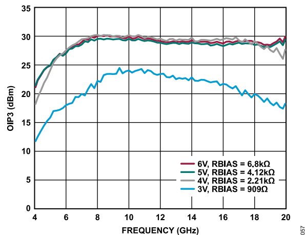
Figure 57. OIP3 vs. Frequency for Various Supply Voltages and R_{BIAS} Values, I_{DQ} = 90\text{ mA}
