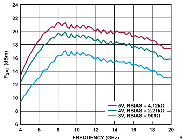
Figure 40. P_{SAT} vs. Frequency for Various Supply Voltages and RBIAS Values, I_{DQ} = 90\text{ mA}
