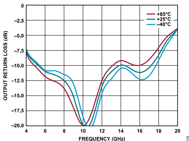
Figure 19. Output Return Loss vs. Frequency for Various Temperatures, 4 GHz to 20 GHz, V_{DD} = 3\text{ V} , I_{DQ} = 90\text{ mA} , R_{BIAS} = 909\ \Omega
