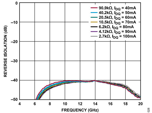
Figure 28. Reverse Isolation vs. Frequency for R_{BIAS} Values and Various I_{DQ} , V_{DD} = 5 V
