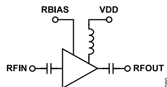
Figure 80. Simplified Schematic
