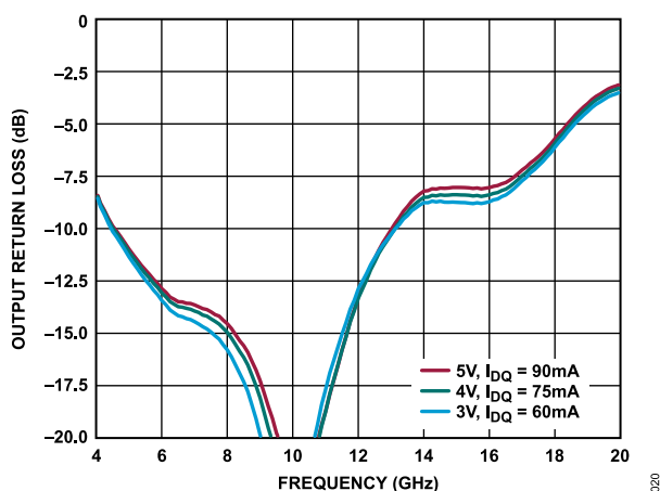
Figure 20. Output Return Loss vs. Frequency for Various Supply Voltages and I_{DQ} , R_{BIAS} = 4.12\text{ k}\Omega
