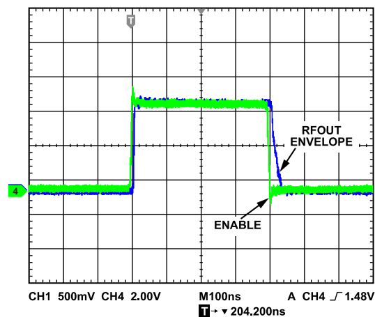
Figure 84. On and/or Off Response of the RF Output Envelope When the IN Pin of the ADG719 Is Pulsed
