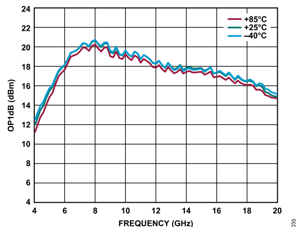
Figure 35. OP1dB vs. Frequency for Various Temperatures, 4 GHz to 20 GHz, V_{DD} = 5\text{ V} , I_{DQ} = 90\text{ mA} , R_{BIAS} = 4.12\text{ k}\Omega
