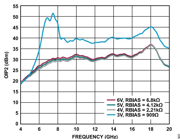
Figure 65. OIP2 vs. Frequency for Various Supply Voltages and R_{BIAS} Values, I_{DQ} = 90\text{ mA}
