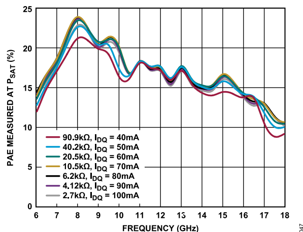
Figure 47. PAE Measured at P_{SAT} vs. Frequency for R_{BIAS} Values and Various I_{DD} , V_{DD} = 5\text{ V}
