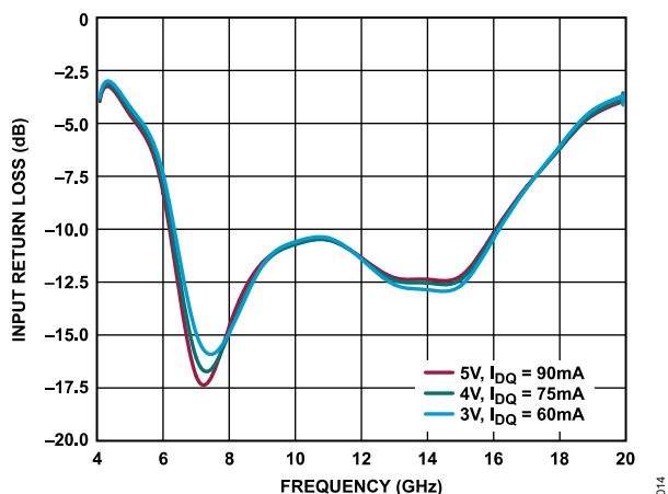
Figure 14. Input Return Loss vs. Frequency for Various Supply Voltages and I_{DQ} , R_{BIAS} = 4.12\text{ k}\Omega
