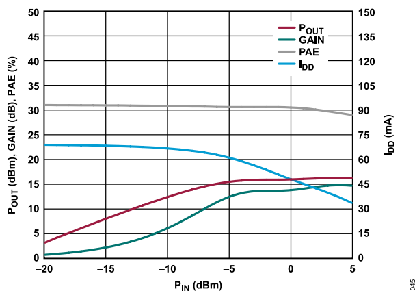
Figure 45. P_{OUT} , Gain, PAE, and I_{DD} vs. P_{IN} , Power Compression at 8 GHz, V_{DD} = 3\text{ V} , R_{BIAS} = 909\text{ }\Omega
