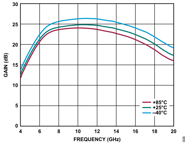
Figure 8. Gain vs. Frequency for Various Temperatures, 4 GHz to 20 GHz, V_{DD} = 3\text{ V} , I_{DQ} = 90\text{ mA} , R_{BIAS} = 909\text{ }\Omega
