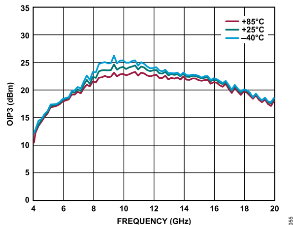
Figure 55. OIP3 vs. Frequency for Various Temperature, 4 GHz to 20 GHz, V_{DD} = 3\text{ V} , I_{DQ} = 90\text{ mA} , R_{BIAS} = 909\ \Omega
