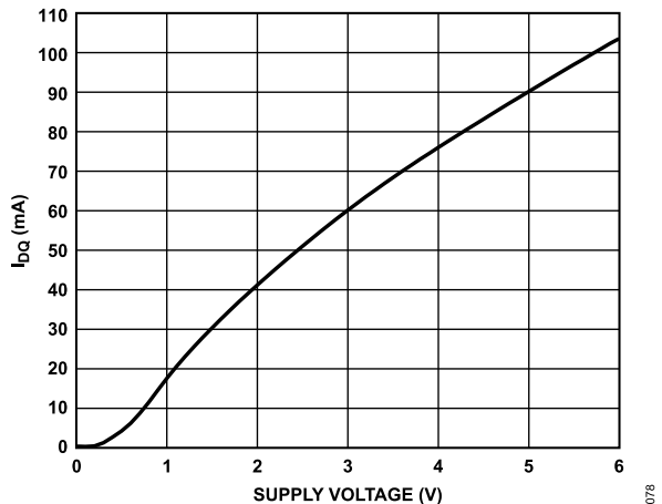
Figure 78. I_{DQ} vs. Supply Voltage, R_{BIAS} = 4.12\ k\Omega
