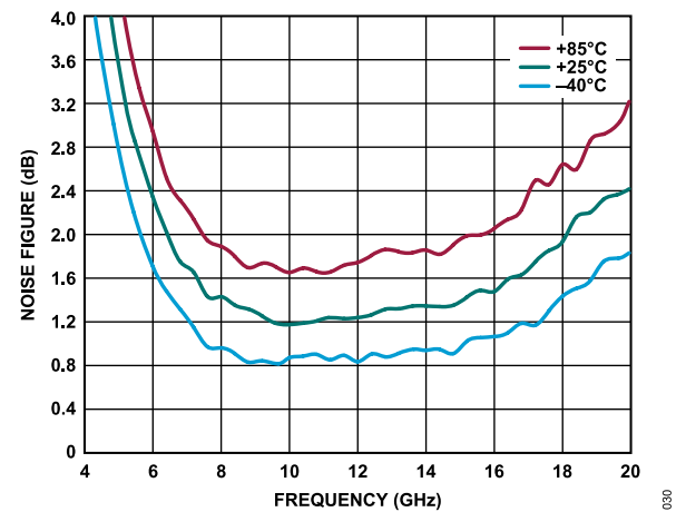
Figure 30. Noise Figure vs. Frequency for Various Temperatures, 4 GHz to 20 GHz, V_{DD} = 5 V, I_{DQ} = 90 mA, R_{BIAS} = 4.12 kΩ
