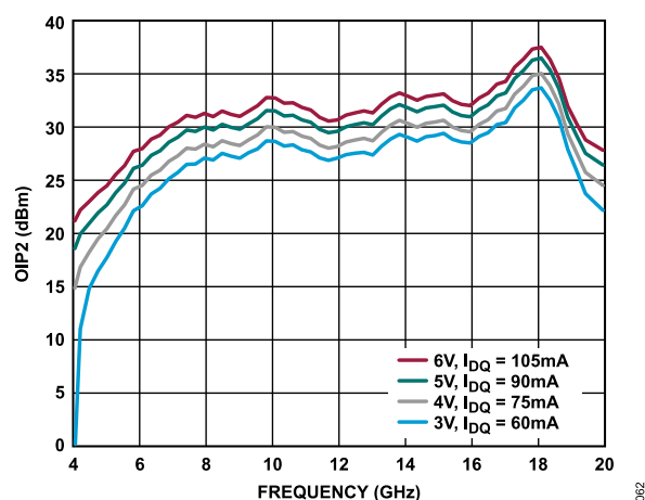
Figure 62. OIP2 vs. Frequency for Various Supply Voltages and I_{DQ} , R_{BIAS} = 4.12\text{ k}\Omega
