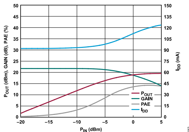
Figure 53. P_{OUT} , Gain, PAE, and I_{DD} vs. P_{IN} , Power Compression at 16 GHz, V_{DD} = 5\text{ V} , R_{BIAS} = 4.12\text{ k}\Omega
