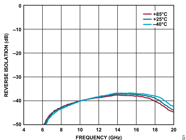
Figure 21. Reverse Isolation vs. Frequency for Various Temperatures, 4 GHz to 20 GHz, V_{DD} = 3\text{ V} , I_{DQ} = 90\text{ mA} , R_{BIAS} = 909\ \Omega
