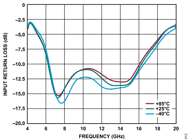
Figure 13. Input Return Loss vs. Frequency for Various Temperatures, 4 GHz to 20 GHz, V_{DD} = 3\text{ V} , I_{DQ} = 90\text{ mA} , R_{BIAS} = 909\ \Omega
