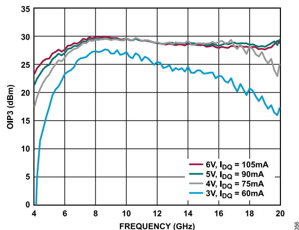
Figure 56. OIP3 vs. Frequency for Various Supply Voltages and I_{DQ} , R_{BIAS} = 4.12\text{ k}\Omega
