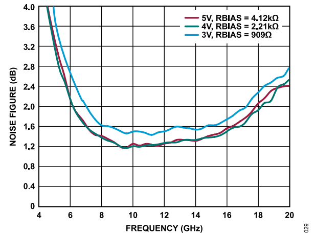
Figure 29. Noise Figure vs. Frequency for Various Supply Voltages and R_{BIAS} Values, I_{DQ} = 90 mA
