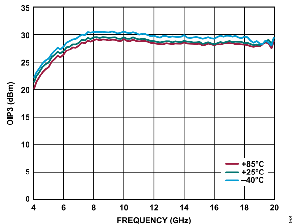
Figure 58. OIP3 vs. Frequency for Various Temperature, 4 GHz to 20 GHz, V_{DD} = 5\text{ V} , I_{DQ} = 90\text{ mA} , R_{BIAS} = 4.12\text{ k}\Omega
