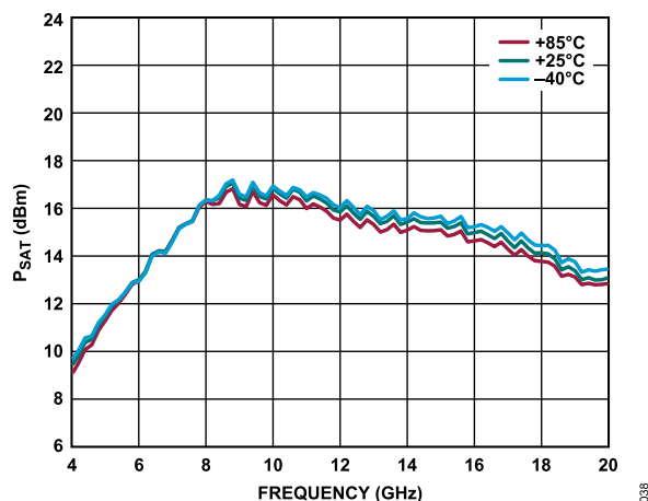
Figure 38. P_{SAT} vs. Frequency for Various Temperatures, 4 GHz to 20 GHz, V_{DD} = 3\text{ V} , I_{DQ} = 90\text{ mA} , RBIAS = 909\text{ }\Omega
