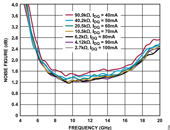
Figure 34. Noise Figure vs. Frequency for R_{BIAS} Values and Various I_{DQ} , V_{DD} = 5\text{ V}
