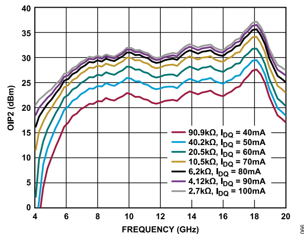
Figure 66. OIP2 vs. Frequency for R_{BIAS} Values and Various I_{DQ} , V_{DD} = 5\text{ V}
