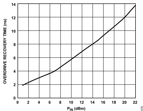
Figure 79. Overdrive Recovery Time vs. P_{IN} at 7 GHz, Recovery to Within 90% of Small Signal Gain Value, V_{DD} = 5 V, R_{BIAS} = 4.12 k \Omega
