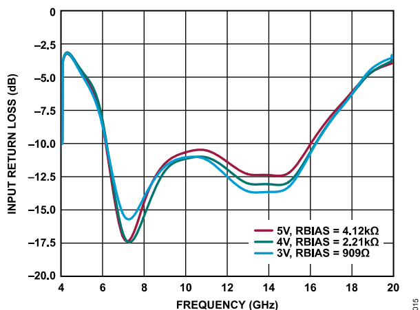
Figure 15. Input Return Loss vs. Frequency for Various Supply Voltages and R_{BIAS} Values, I_{DQ} = 90\text{ mA}
