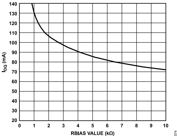
Figure 74. I_{DQ} vs. R_{BIAS} Value, 1\ \Omega to 10\ k\Omega , V_{DD} = 5\ V
