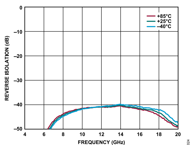
Figure 24. Reverse Isolation vs. Frequency for Various Temperatures, 4 GHz to 20 GHz, V_{DD} = 5\text{ V} , I_{DQ} = 90\text{ mA} , R_{BIAS} = 4.12\text{ k}\Omega
