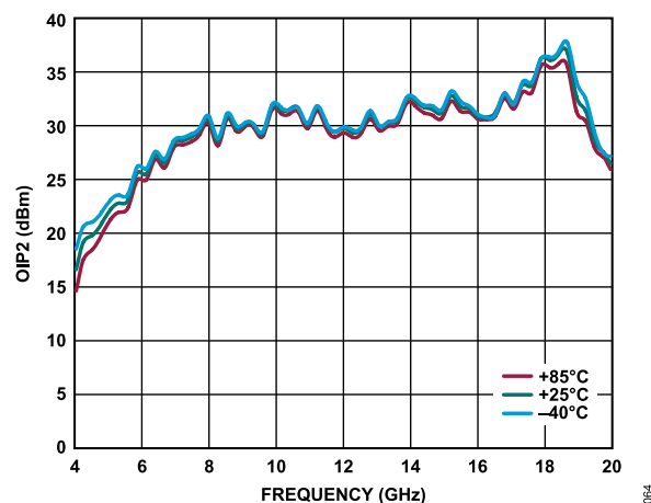
Figure 64. OIP2 vs. Frequency for Various Temperature, 4 GHz to 20 GHz, V_{DD} = 5\text{ V} , I_{DQ} = 90\text{ mA} , R_{BIAS} = 4.12\text{ k}\Omega
