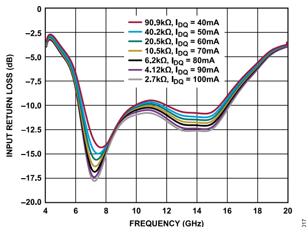
Figure 17. Input Return Loss vs. Frequency for R_{BIAS} Values and Various I_{DQ} , V_{DD} = 5\text{ V}
