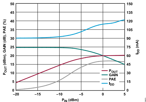
Figure 52. P_{OUT} , Gain, PAE, and I_{DD} vs. P_{IN} , Power Compression at 12 GHz, V_{DD} = 5\text{ V} , R_{BIAS} = 4.12\text{ k}\Omega
