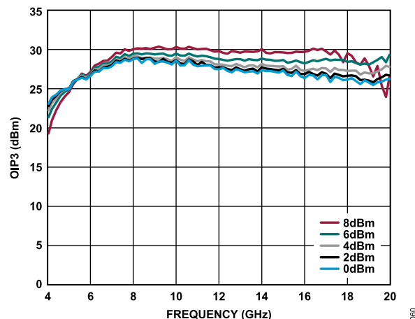
Figure 60. OIP3 vs. Frequency for Various P_{OUT} per Tone, 4 GHz to 20 GHz, V_{DD} = 5\text{ V} , I_{DQ} = 90\text{ mA} , R_{BIAS} = 4.12\text{ k}\Omega
