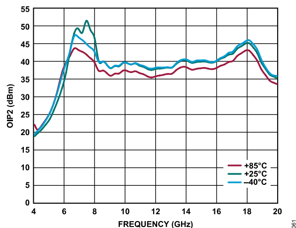
Figure 61. OIP2 vs. Frequency for Various Temperature, 4 GHz to 20 GHz, V_{DD} = 3\text{ V} , I_{DQ} = 90\text{ mA} , R_{BIAS} = 909\ \Omega
