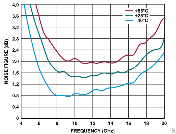
Figure 27. Noise Figure vs. Frequency for Various Temperatures, 4 GHz to 20 GHz, V_{DD} = 3 V, I_{DQ} = 90 mA, R_{BIAS} = 909 Ω
