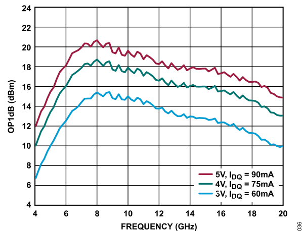
Figure 36. OP1dB vs. Frequency for Various Supply Voltages and I_{DQ} , R_{BIAS} = 4.12\text{ k}\Omega
