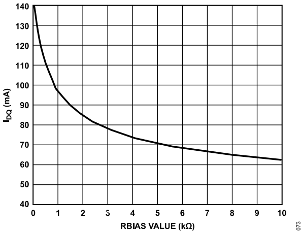
Figure 73. I_{DQ} vs. R_{BIAS} Value, 1\ \Omega to 10\ k\Omega , V_{DD} = 3\ V
