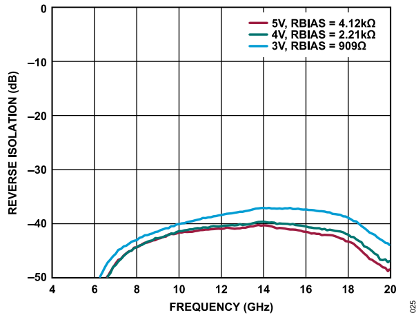
Figure 25. Reverse Isolation vs. Frequency for Various Supply Voltages and R_{BIAS} Values, I_{DQ} = 90 mA
