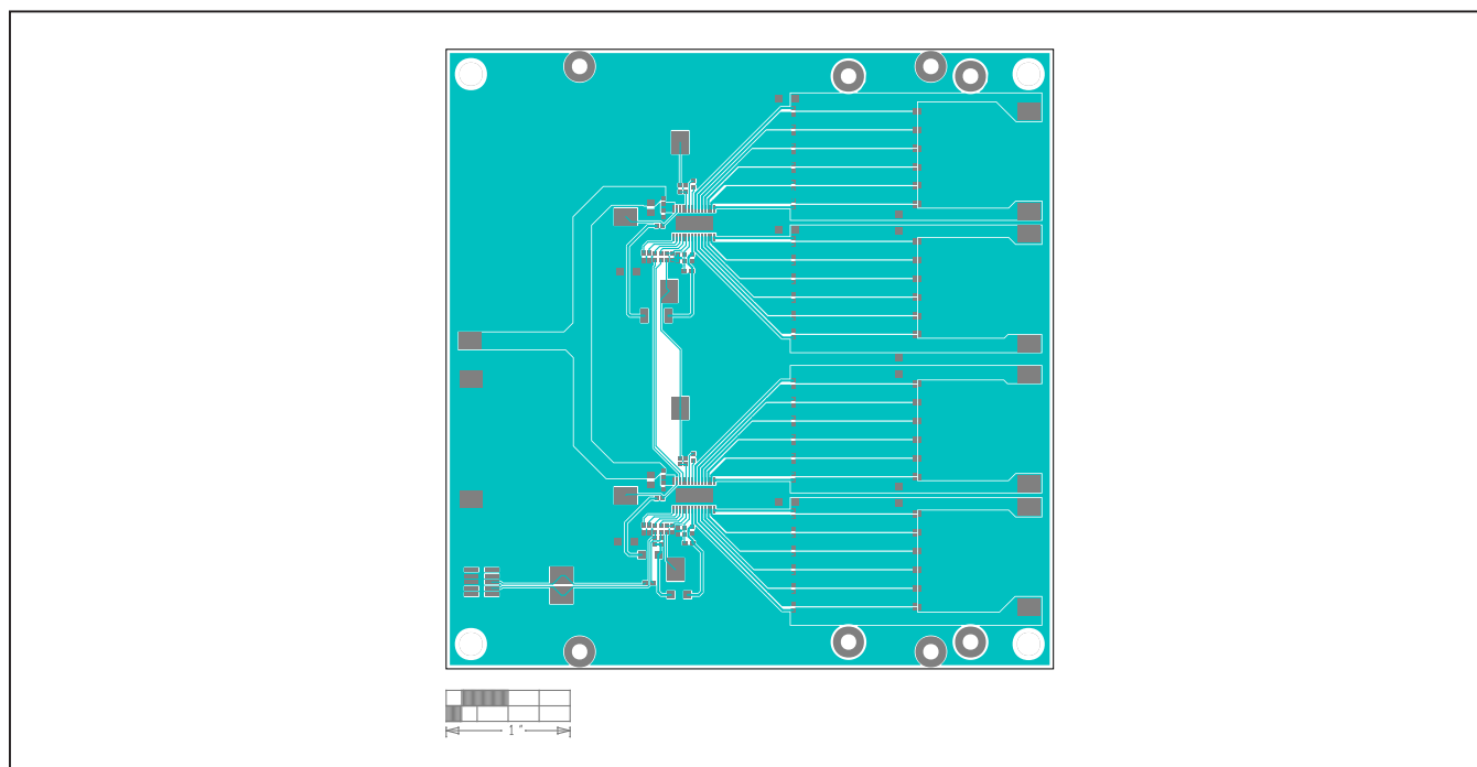
MAX25608 EV Kit PCB Layout—Top View
