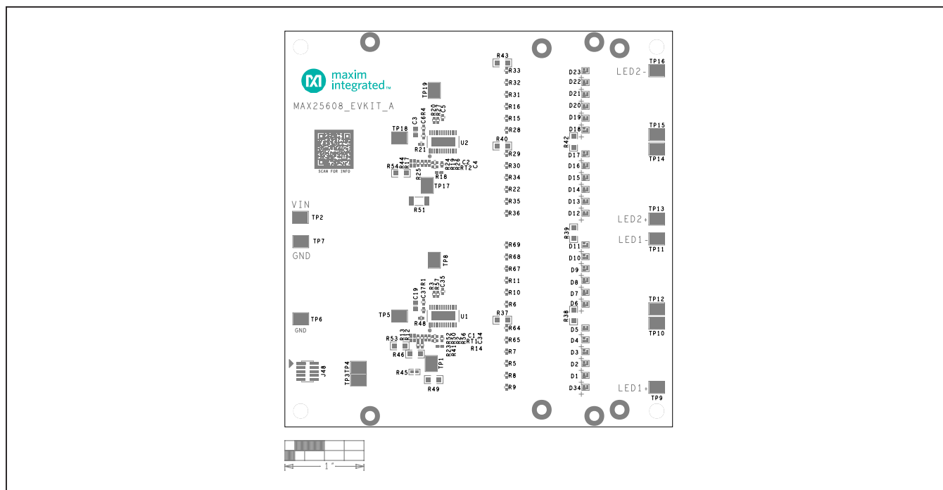
MAX25608 EV Kit Component Placement Guide—Top Silkscreen
