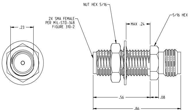
CGM-1180-FB-SMA-00
