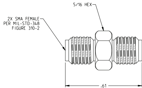
CGM-1180-FF-SMA-09
