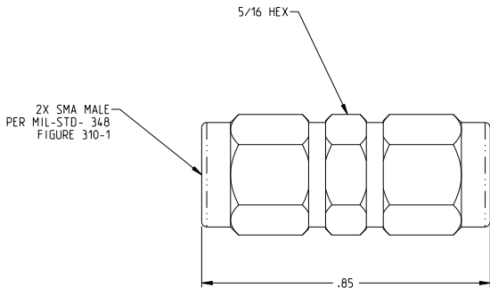
CGM-1180-MM-SMA-09
