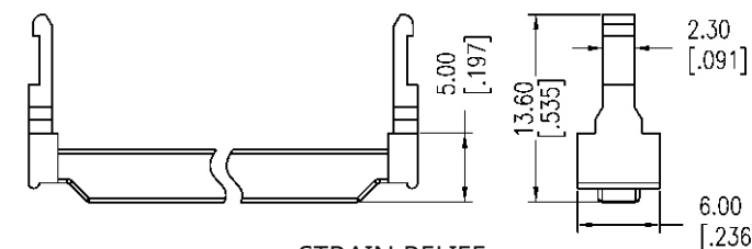
STRAIN RELIEF
