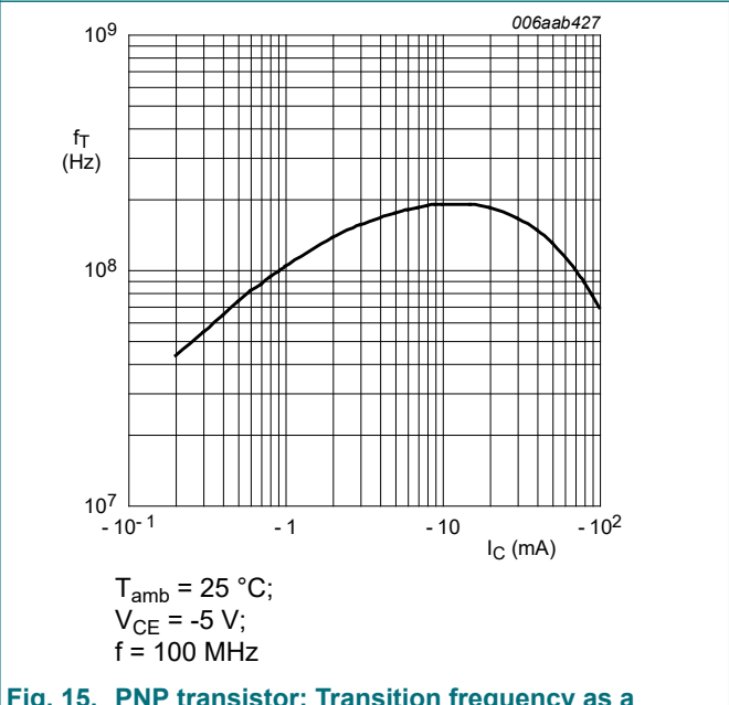
Fig. 15. PNP transistor: Transition frequency as a function of collector current; typical values
