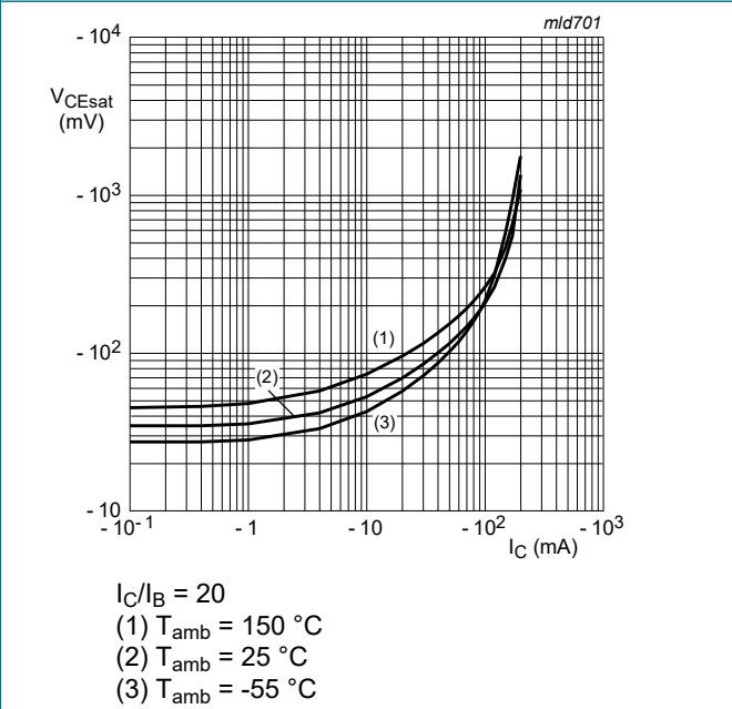
Fig. 14. PNP TR2: Collector-emitter saturation voltage as a function of collector current; typical values
