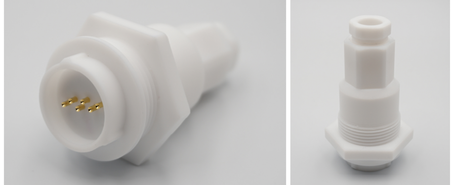
MP6-PM-F-RTD2 Panel mount connector – female, 6 sockets
