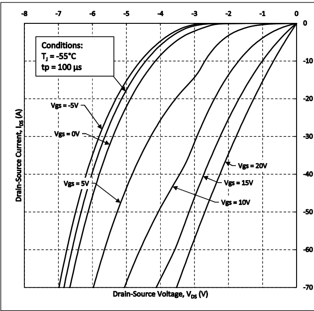
Figure 9. Freewheeling Diode Characteristics at T_J = -55 °C
