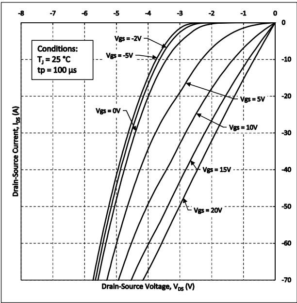
Figure 10. Freewheeling Diode Characteristics at T_J = 25 °C
