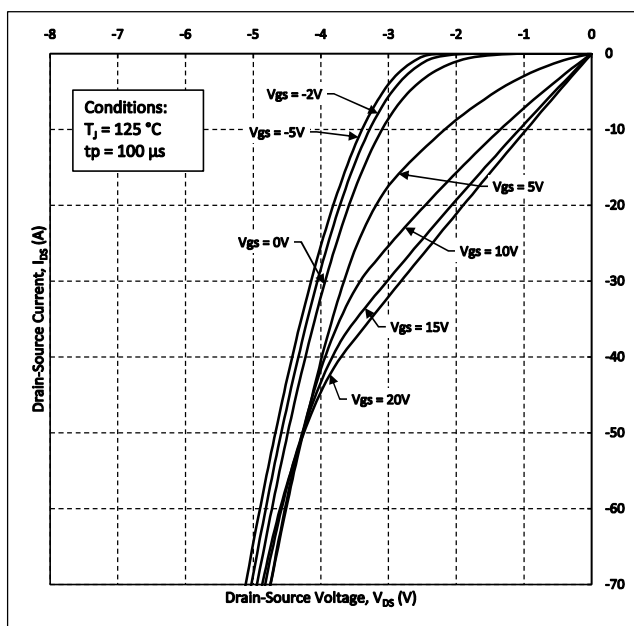
Figure 11. Freewheeling Diode Characteristics at T_J = 125^\circ\text{C}
