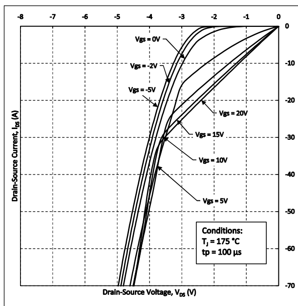
Figure 12. Freewheeling Diode Characteristics at T_J = 175^\circ\text{C}
