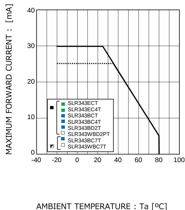
Fig.4 Derating
