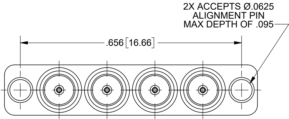
ALIGNMENT PIN INFORMATION
