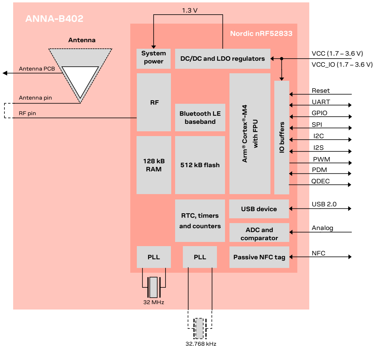
Figure 1: Block diagram of ANNA-B402
