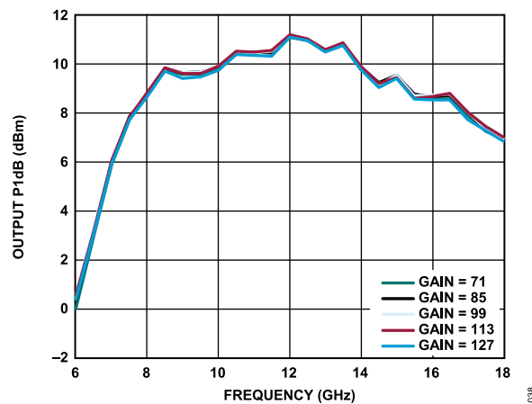
Figure 43. Output P1dB vs. Frequency over Gain, Transmit Channel
