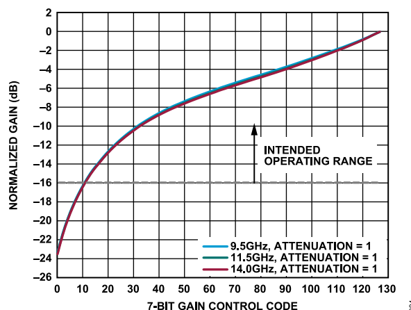
Figure 95. Normalized Gain vs. 7-Bit Gain Control Code
