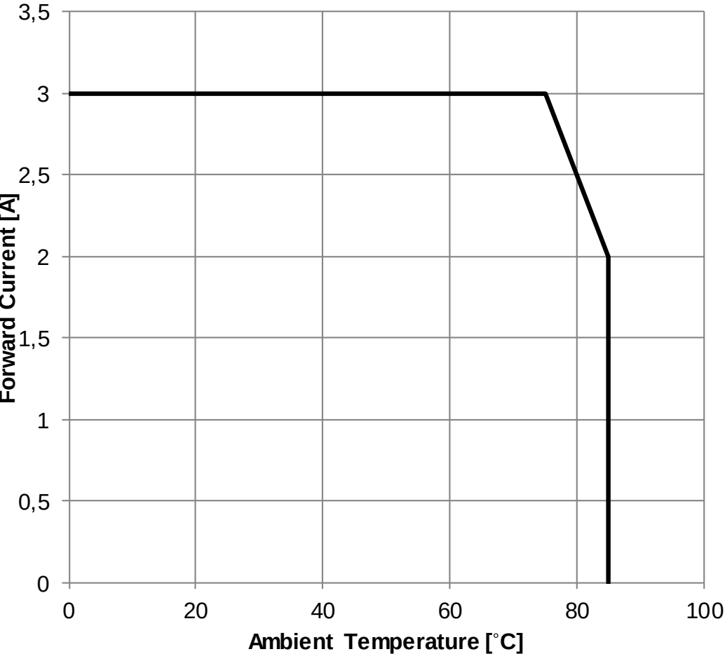
Derating Curve:
