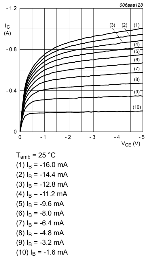
Fig. 7. BC807-16W-Q: Collector current as a function of collector-emitter voltage; typical values
