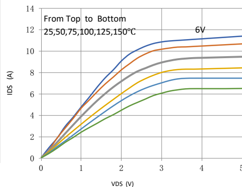
I_{ds} - V_{ds} curves @ V_{gs}=6V & different Temperatures
