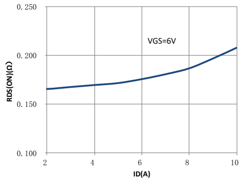
I_{ds} - R_{ds(on)} Curve
