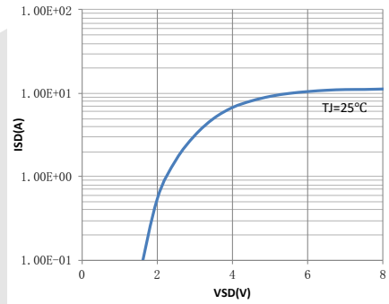
I_{sd} - V_{sd} curve @ 25°C
