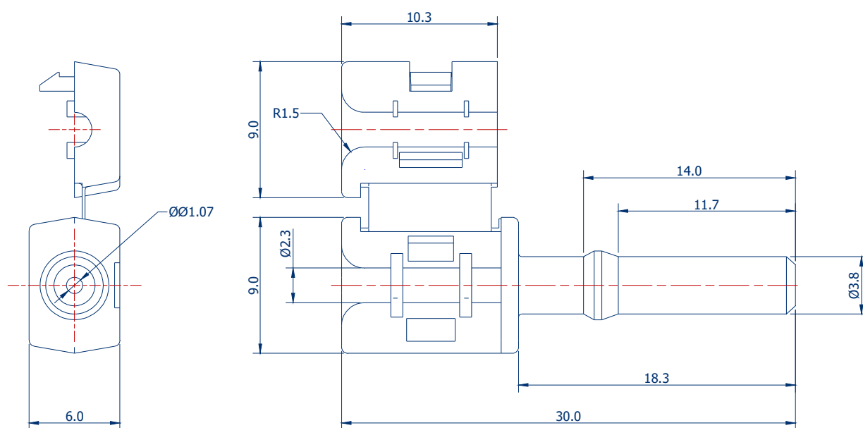
Figure 4. Mechanical Dimensions
