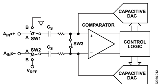
Figure 25. ADC Acquisition Phase
