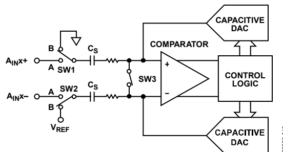
Figure 26. ADC Conversion Phase
