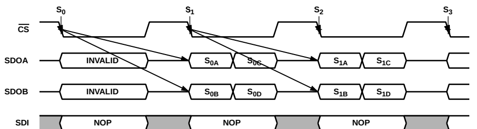
Figure 37. Reading Conversion Results, 2-Wire Mode
