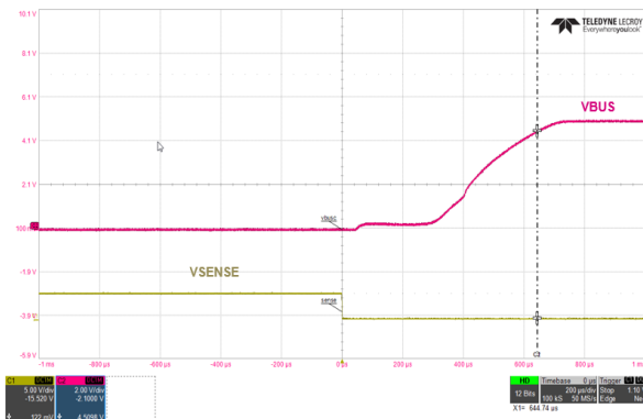
Figure 5. VBUS turn-on time ( T_{ON} )
