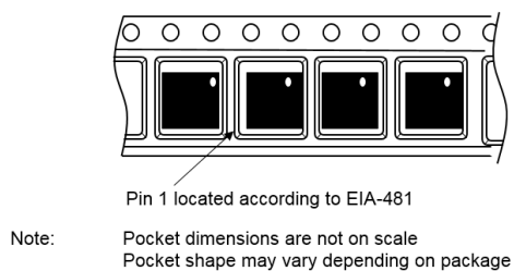
Figure 20. Package orientation in reel
