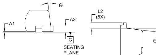
DETAIL "B"
