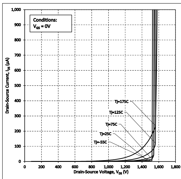
Figure 12. I_{DSS} vs. Temperature
