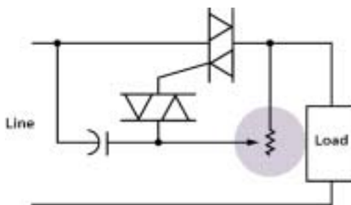
Figure 14: Triac Control Circuit
