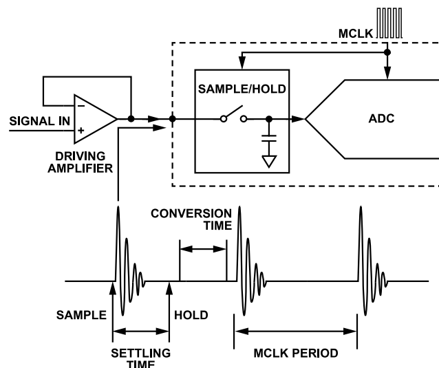
Figure 60. Driving the Input of a Discrete Time ADC
