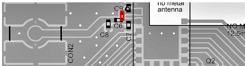
Figure 4: Capacitor connection to internal antenna
