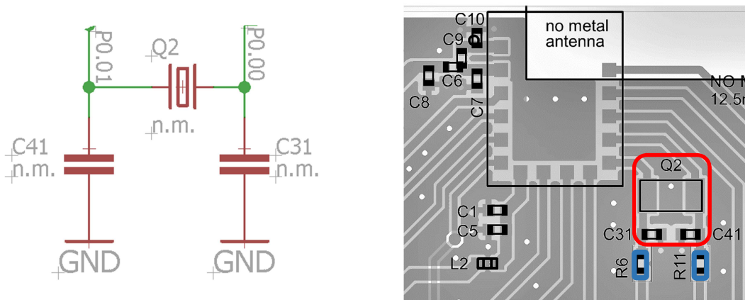
Figure 7: LFXO mounting
