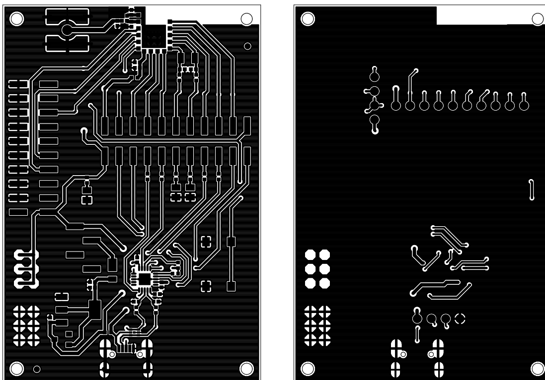
Figure 9: Top layer (top), bottom layer (bottom)
