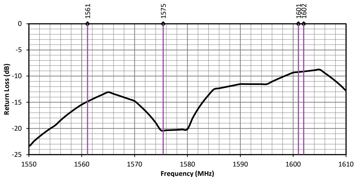
Figure 3. ANT-GNCP-C257L160 Return Loss
