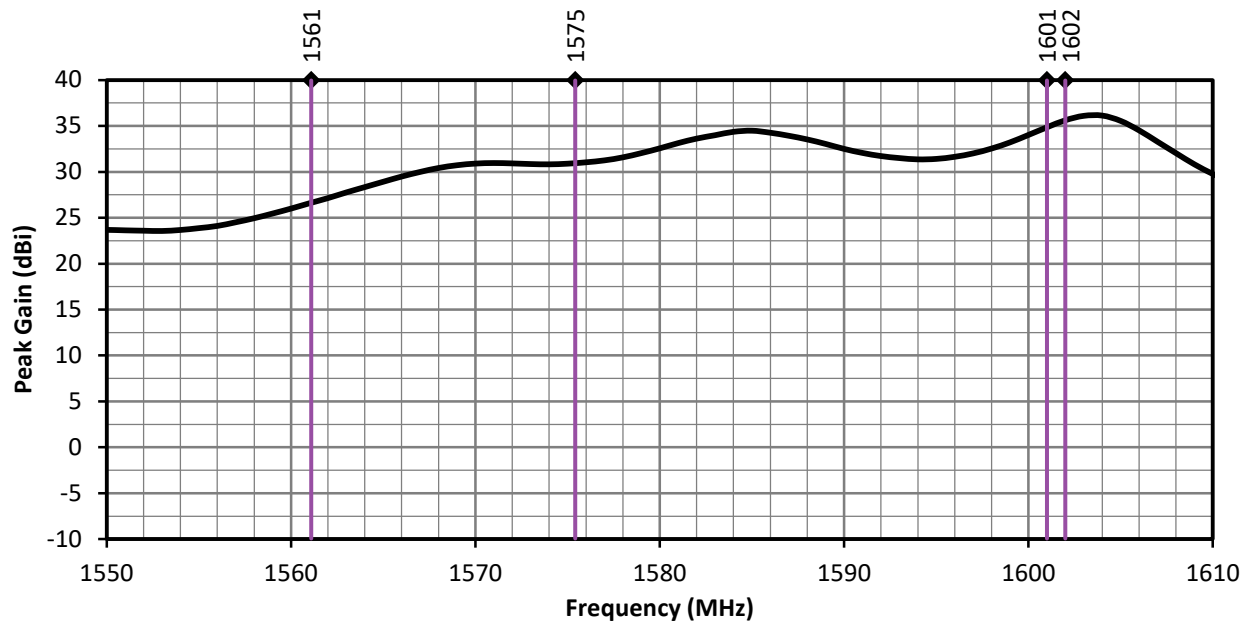
Figure 4. ANT-GNCP-C257L160 Peak Gain
