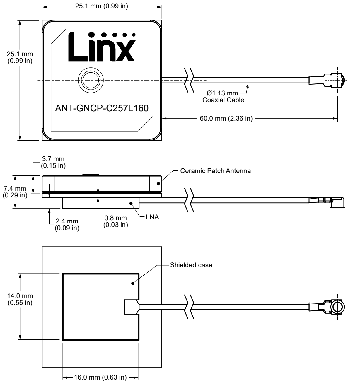
Figure 1. ANT-GNCP-C257L160 Antenna Dimensions
